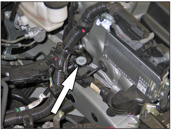
16. Remove the air box mounting grommet shown.
