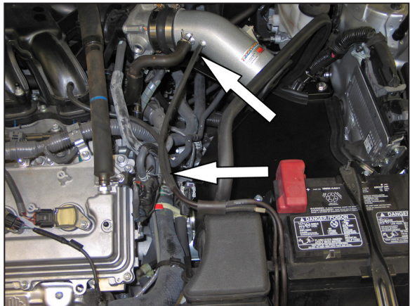
37. Connect the shorter provided vacuum line to the open factory union fitting and then connect the open end to the K&N® intake tube.
