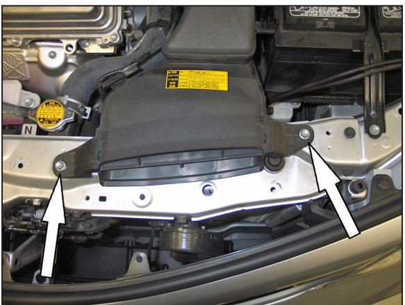
13. Remove the two bolts securing the fresh air duct and then remove the fresh air duct from the vehicle.
