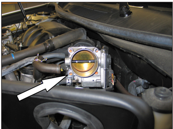
27. Remove the front lower throttle body mounting bolt shown. NOTE: This bolt will be reused in the next step.
