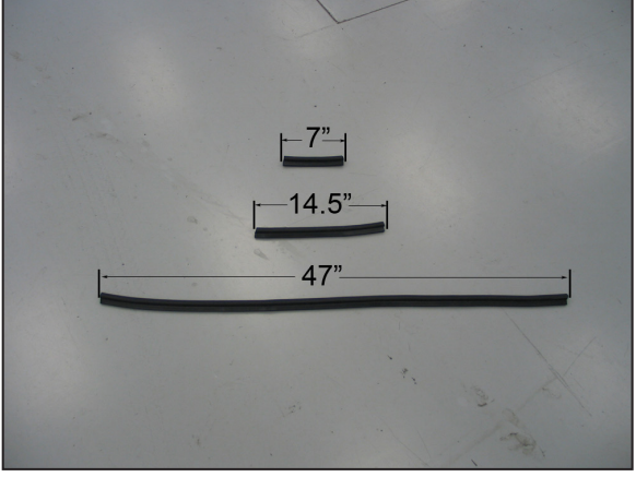
19. Cut the provided edge trim into three sections, the long section is 47" long, the medium section is 14-1/2" long, the short section is 7" long.
