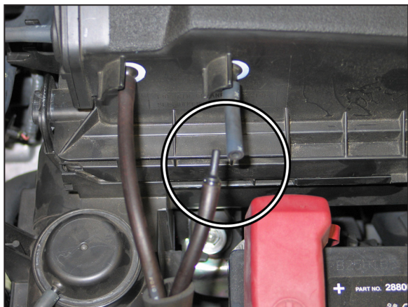
7. Disconnect the vacuum line from the union fitting shown leaving the union installed into the vacuum line attached to the vehicle.
