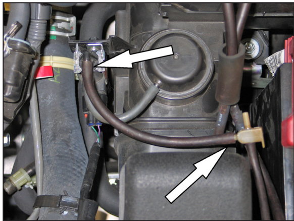
9. Remove the vacuum hose shown from the TEE fitting and vacuum switching valve.
