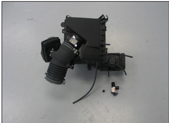
23. Remove the vacuum switching valve from the air box as shown.
