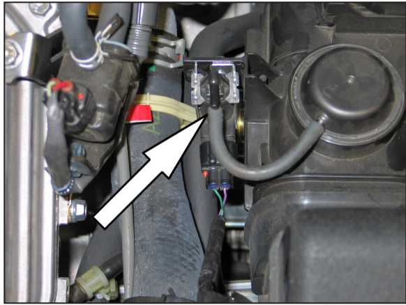
10. Disconnect the lower vacuum hose from the vacuum switching valve.
