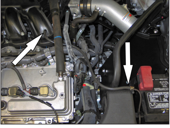
36. Install the provided longer vacuum hose to the vacuum TEE and install the open end onto the intake plenum.
