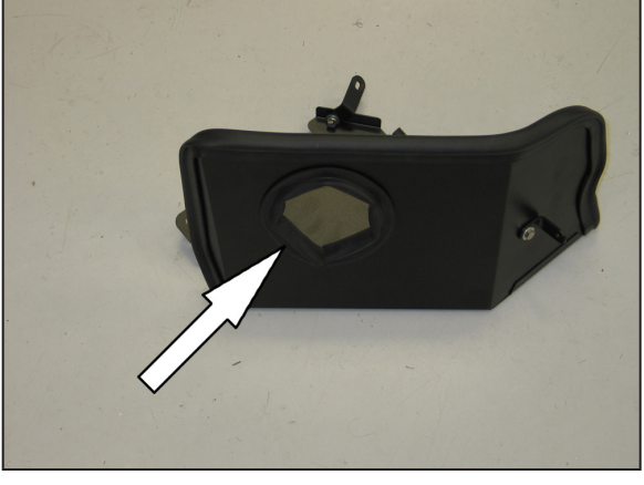
21. Install the 14.5" length edge trim into the hole of the heat shield as shown.
