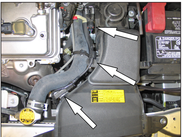
12. Disconnect the vacuum switch electrical connection and then unhook the harness from the fresh air duct.
