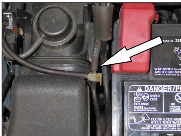
8. Disconnect the vacuum line at the TEE fitting shown.
