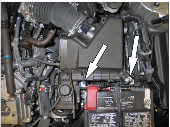
14. Remove the two bolts shown securing the air box.
