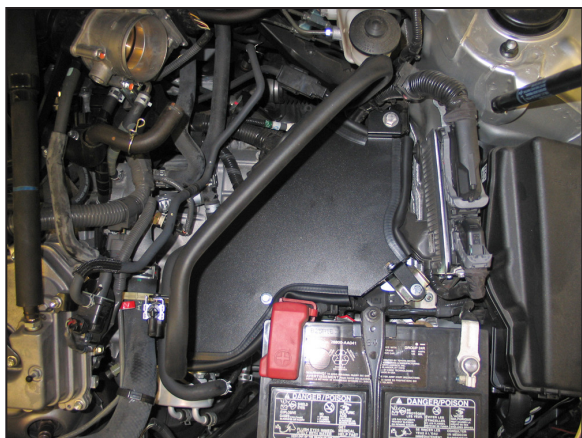
26. Set the heat shield into position and secure with the provided hardware.
