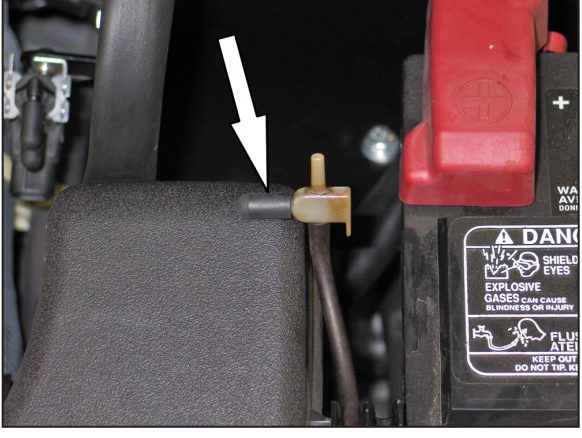
35. Install the provided vacuum plug onto the vacuum TEE.
