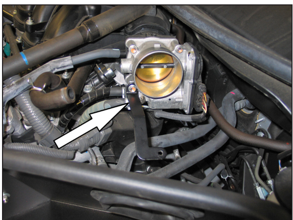
28. Install the tube mounting bracket (06485) onto the throttle body securing with the factory bolt removed in the previous step. NOTE: Do not completely tighten at this time.
