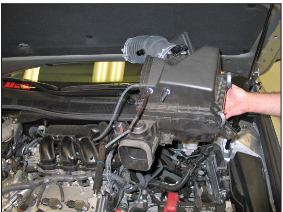
15. Remove the air box from the vehicle. NOTE: K&N Engineering, Inc., recommends that customers do not discard factory air intake.
