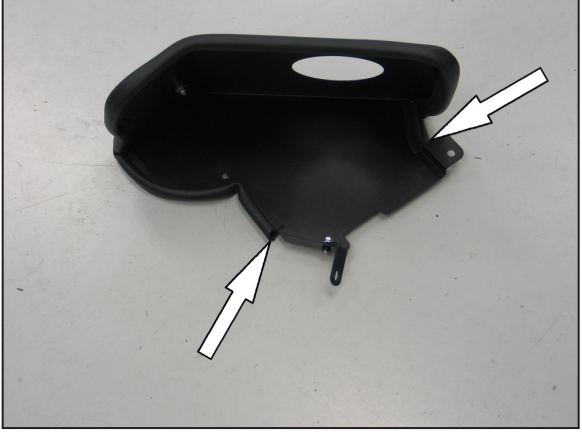
20. Install the 47" long section of edge trim onto the heat shield as shown.
