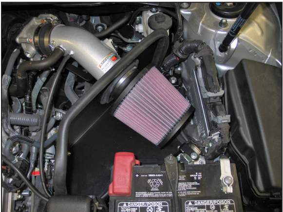
41. Install the K&N® air filter and secure with the provided hose clamp.
