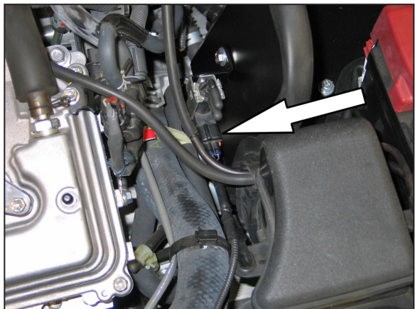
38. Reconnect the vacuum switching valve electrical connection and secure the wiring harness to the fresh air intake scoop.
