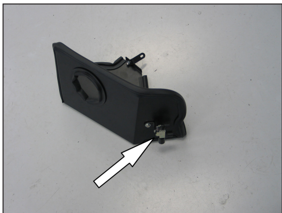
24. Secure the vacuum switching valve to the "L" installed onto the heat shield as shown and then install the provided vacuum caps.
