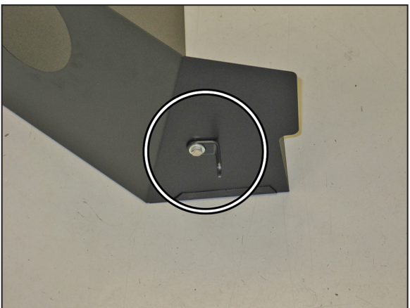
17. Install the heat shield mounting bracket (070066) onto the heat shield using the provided hardware. NOTE: The slotted end of the bracket attaches to the heat shield.
