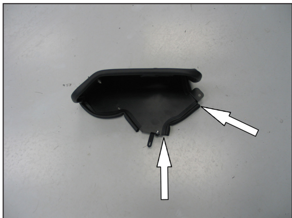
22. Install the 7" section of edge trim onto the heat shield as shown.
