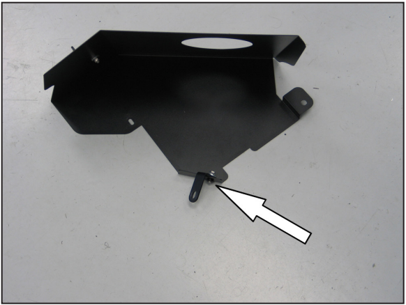
18. Install the heat shield mounting bracket (070812) onto the heat shield using the provided hardware. NOTE: Do not completely tighten at this time.
