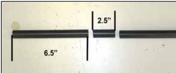
27. Using a knife, cut the provided silicone hose in 2.5" and 6.5" pieces as shown.
