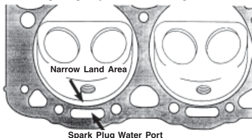
Lightweight Cylinder Head Casting Outline
