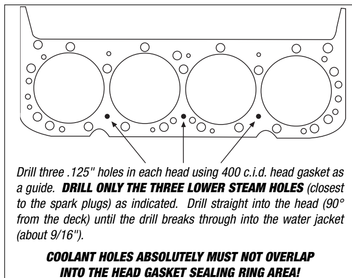
Figure 1 - Steam Hole Locations (400 C.I.D. Engines ONLY) IMPORTANT NOTICE
