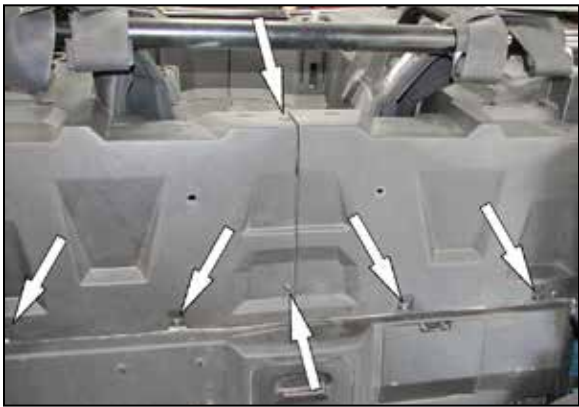
12. Reinstall six of the eight bolts removed in step #3. Reinstall the seats. NOTE: the two upper air filter housing bolts will not be reused and the locations left blank.
