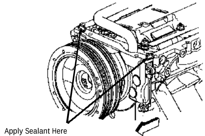
Figure 3 - Sealant Locations
