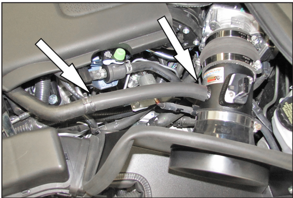
22. Install the crank case vent hose onto the fitting on the K&N intake tube and the install the hose mender into the factory crank case vent hose and secure with the factory spring clamp.
