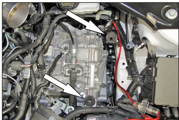
7. Remove the two air box mounting grommets shown from the mounting brackets.
