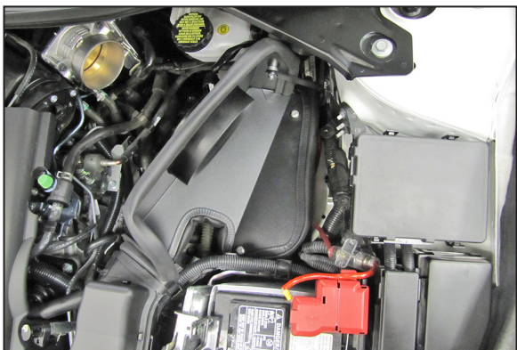
14. Install the heat shield assembly onto the rubber mounted studs. Secure the heat shield with the provided hardware. Clip the transmission vent into the hole in the heat shield. NOTE: Do not secure the mounting bracket at this time.
