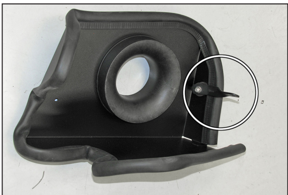
13. THIS STEP IS FOR THE NISSAN PATHFINDER AND INFINTI JX35 VEHICLES ONLY. Install the heat shield mounting bracket (07947) onto the heat shield as shown using the male/male rubber mounted stud and hardware.
