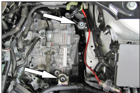
8. Install the two provided rubber mounting studs onto the air box mounting brackets as shown. NOTE: The forward rubber mounted stud should be a 1" tall, male/ female; the rear rubber mounted stud should be a 1/2" tall male/ female. Be sure to use two fender washers and one rubber washer on each rubber mounted stud. The fender washers will be on each side of the bracket with the rubber washer sandwiched between.
