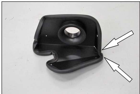
11. Install the provided edge trim on to the heat shield as shown. NOTE: Some trimming of the edge trim will be necessary.
