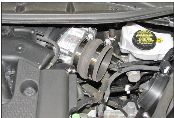
15. Install the provided hump hose (08171) onto the throttle body and secure with provided hose clamp.
