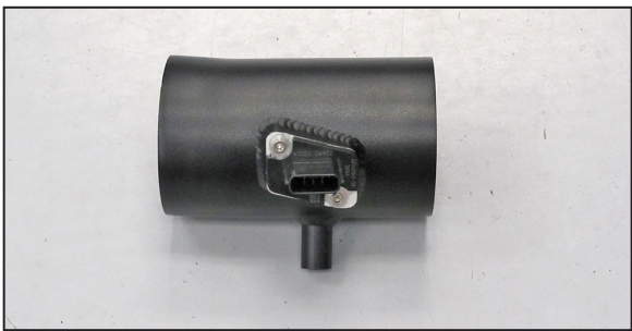
18. Install the mass air sensor into the K&N intake tube and secure with the provided hose clamp.
