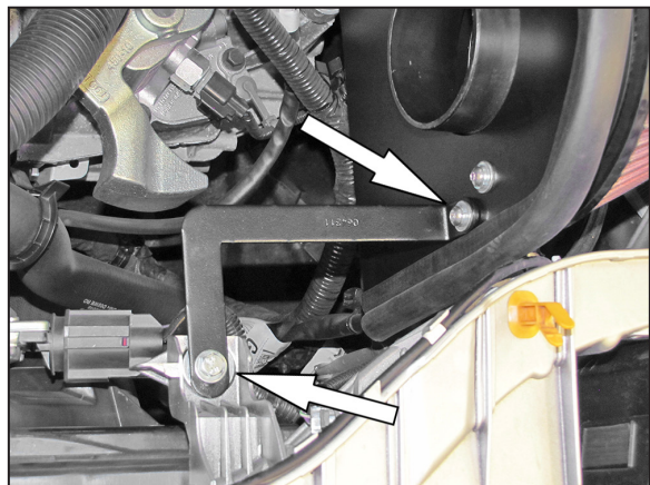
13. Install the heat shield mounting bracket (064311) onto the heat shield and core support with the provided hardware.
