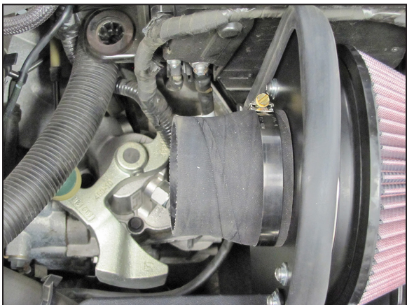
15. Install the provided coupling hose #084055 onto the filter adapter as shown and secure with the provided hose clamp.
