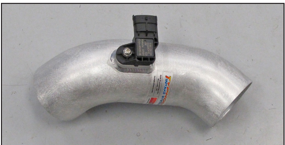
17. Install the pressure sensor into the K&N® intake tube and secure with the provided hardware.
