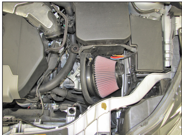
12. Install the K&N® air filter onto the filter adapter and secure with the provided hose clamp.
