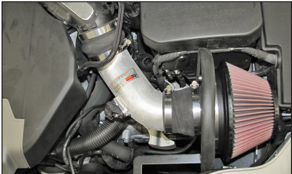
18. Install the K&N® intake tube into the hose at the plenum and then into the hose at the filter adapter and then secure with the provided hose clamps.
