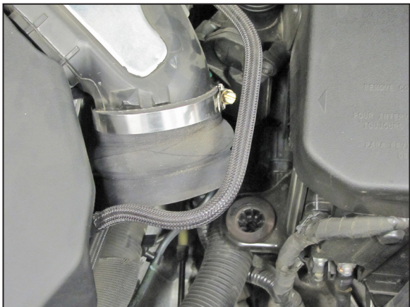
14. Install the coupling hose #08696 onto the plenum and secure with the hose clamp.
