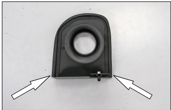
10. Install the provided edge trim onto the heat shield as shown. NOTE: Some trimming of the edge trim will be necessary.
