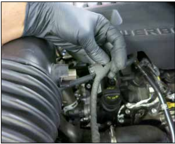
3. Disconnect the IAT sensor electrical connection.
