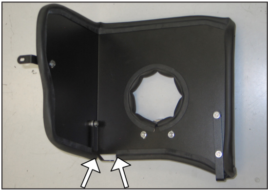
17. Install the provided longer edge trim onto the heat shield as shown. NOTE: Trimming of the edge trim will be necessary.
