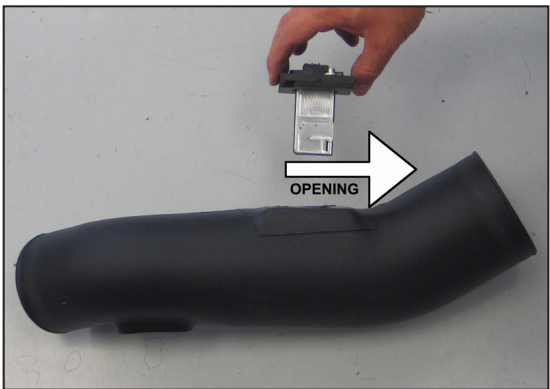
23. Install the mass air sensor assembly into the K&N® intake tube as shown using the provided hardware. NOTE: Ensure the opening is pointed towards the filter end of the intake tube.
