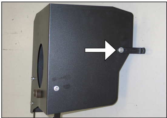
14. Install the provided heat shield mounting bracket (070742) onto the heat shield using the provided hardware and spacer as shown.
