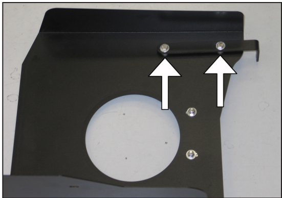
12. Install the heat shield mounting bracket (070902) onto the heat shield as shown using the provided spacers and hardware.
