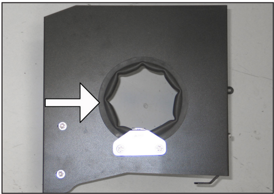
16. Install the provided shorter edge trim into the hole of the heat shield as shown. NOTE: Trimming of the edge trim will be necessary.
