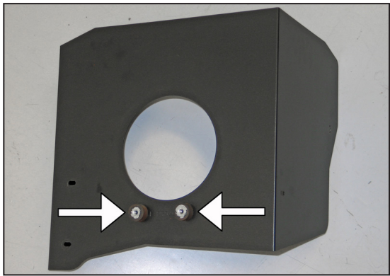
11. Install the two rubber mounted studs onto the heat shield as shown using the provided hardware.
