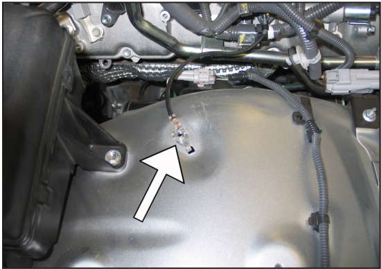
18. Remove the bolt that secures the ground strap to the inner fender. NOTE: This bolt will be reused.
