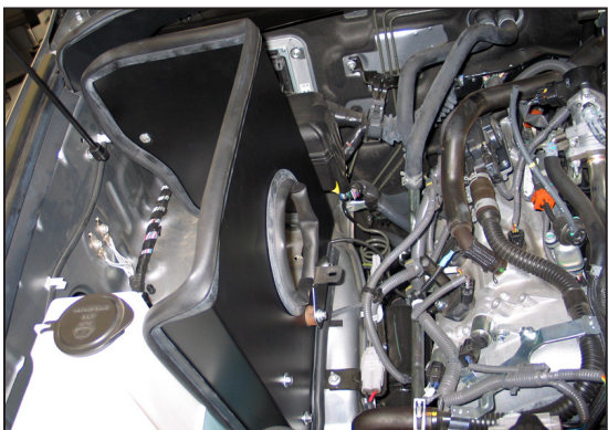
19. Set the heat shield into position on the inner fender and then secure with the factory bolt removed in step #18 with the provided hardware. NOTE: Ensure the ground strap is between the mounting bracket and inner fender.
