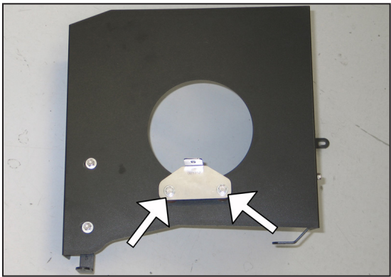
15. Install the tube mounting bracket (083152) onto the rubber mounted studs as shown using the provided hardware.
