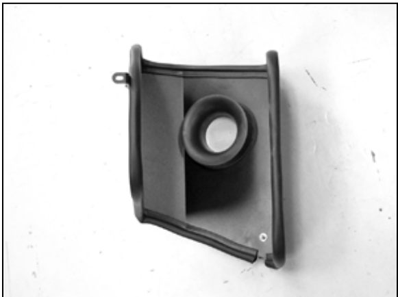
14. Install the provided edge trim onto the heat shield as shown. NOTE: Some trimming of the edge trim will be necessary.
