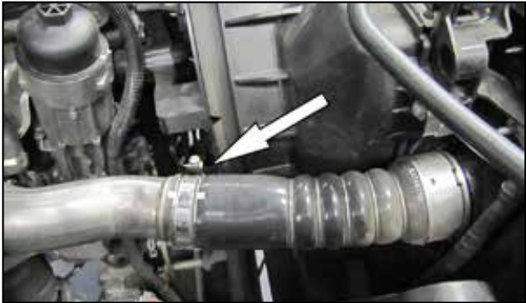
8. Pull the intake tube forward and then disconnect the vent tube quick disconnect and then remove the intake tube from the vehicle.
