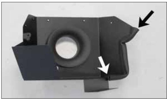
18. Install the 10.5" long piece onto the heat shield as shown.
