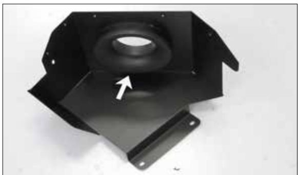
14. Install the filter adapter into the heat shield and secure with the provided hardware.
