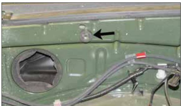
13. Install the 6mm rubber mounted stud into the inner fender location shown. NOTE: On some models, a horn may be attached in this location.
