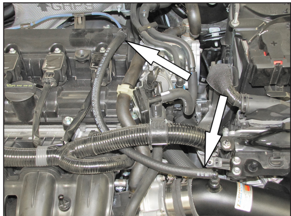
22. Install the provided crank case vent hose onto the valve cover port and then onto the 90° fitting in the intake tube. NOTE: Some trimming of the hose may be necessary.
