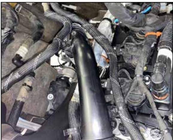
26. Resecure the coolant hoses to the hot-side charge tube.
