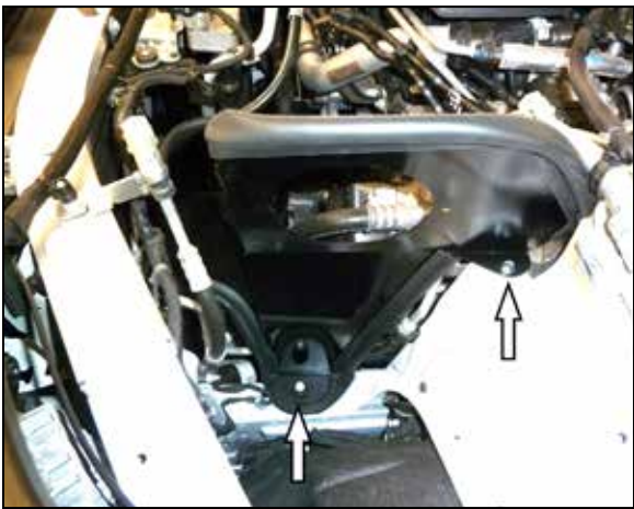
11. Install the heat shield into the vehicle so that the mounting stud inserts into the grommet in the heat shield then secure to the inner fender with the provided bolt.
