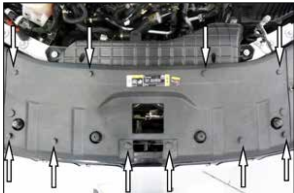
5. Remove the ten retaining clips that secure the radiator cover and then remove the cover from the vehicle.
