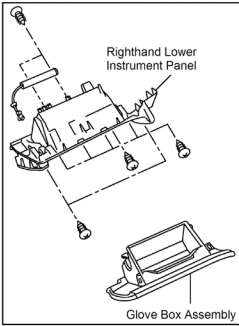
Fig. 1 Instrument lower panel removal. 2010-13 Nissan 370Z
