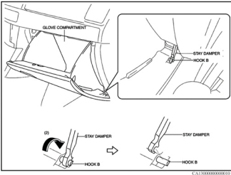
Fig. 1 Glove compartment removal (Part 2 of 3). 2013 Mazda CX-5
