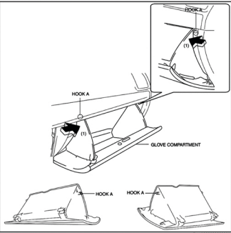
Fig. 1 Glove compartment removal (Part 1 of 3). 2013 Mazda CX-5
