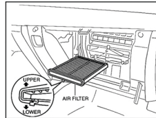
Fig. 2 Cabin air filter removal. 2013 Mazda CX-5
