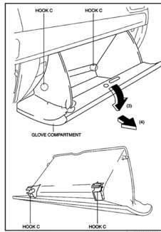
Fig. 1 Glove compartment removal (Part 3 of 3). 2013 Mazda CX-5
