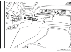
Fig. 11 Passenger compartment air filter removal. 2013 Cadillac XTS
