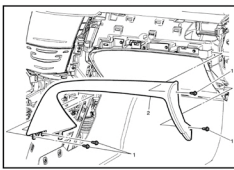
Fig. 4 Lower trim panel removal. 2013 Cadillac XTS
