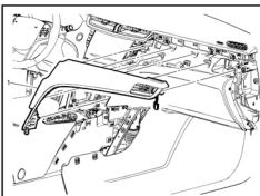
Fig. 3 Upper trim panel removal. 2013 Cadillac XTS
