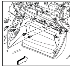
Fig. 8 Instrument panel compartment lower fastener removal. 2013 Cadillac XTS
