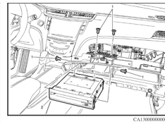
Fig. 9 Video disc player control removal. 2013 Cadillac XTS
