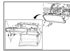
Fig. 10 Instrument panel compartment shelf removal. 2013 Cadillac XTS
