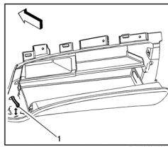
Fig. 6 Instrument panel compartment door damper disconnection. 2013 Cadillac XTS
