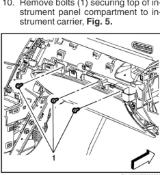
Fig. 5 Instrument panel compartment upper fastener removal. 2013 Cadillac XTS
