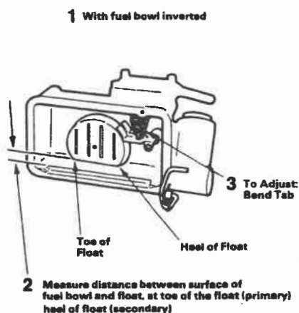
Non-Adjustable Type Dry Float Setting FIGURE 1
