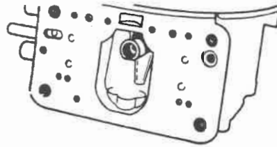
Type B Main body has accelerating pump passage boss recessed .20 (almost 1/4") below gasket face and use connector tube and "O" rings.
