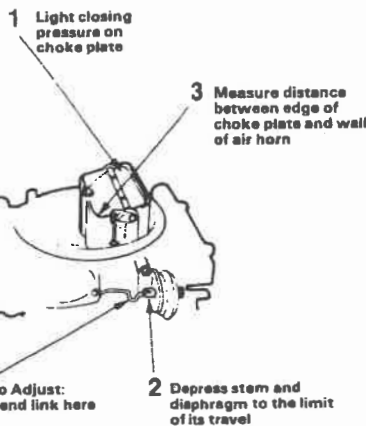
Choke Qualifying (Vacuum Pull Down) Adjustment FIGURE 10
