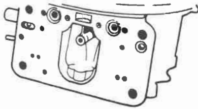
Type A Main body has accelerating pump passage boss flush, or even, with gasket surface for metering body.
