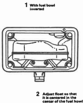
Center Inlet Type Dry Float Setting FIGURE 2
