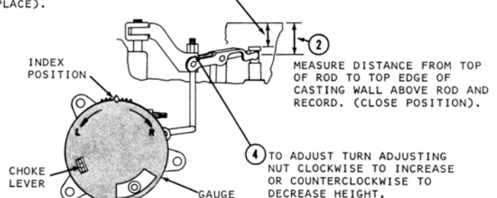
COLD ENRICHMENT METERING ROD ADJUSTMENT
