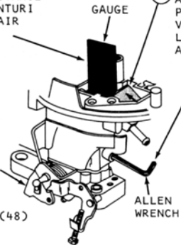
VENTURI VALVE LIMITER ADJUSTMENT.
